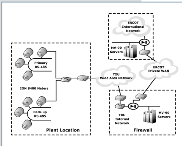
Diagram of the ERCOT-polled settlement meter communication scheme.
